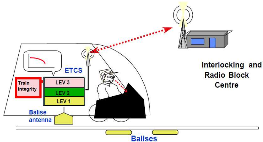
Figure 21: ETCS – Level 3 operational diagrams
