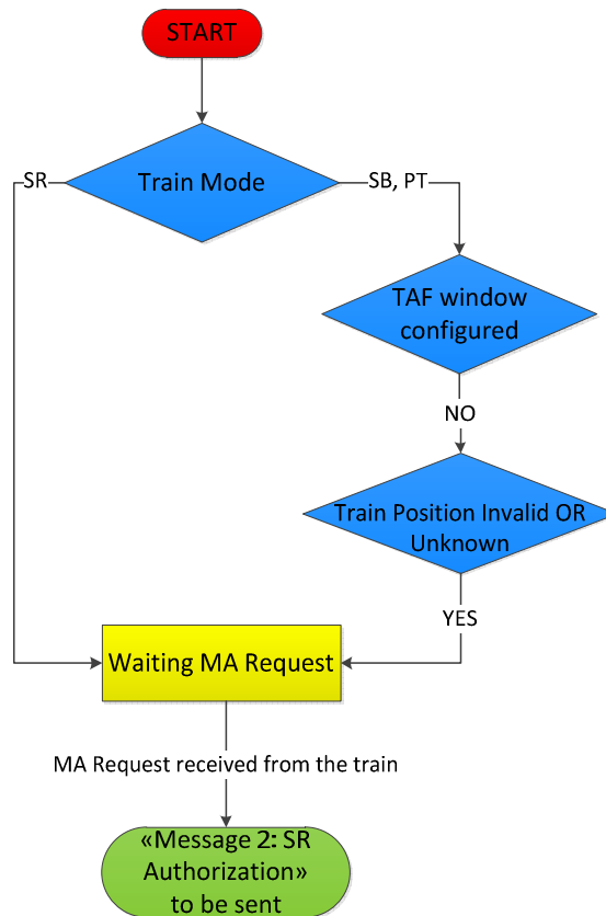
Figure 42: Triggering functions for “Message 2: SR Authorization”
