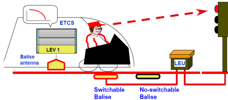
Figure 17: ETCS – Level 1 operation diagram
