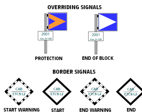
Figure 18: indicator panels
