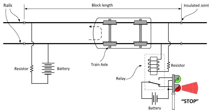
Figure 4: track circuit with occupied block
