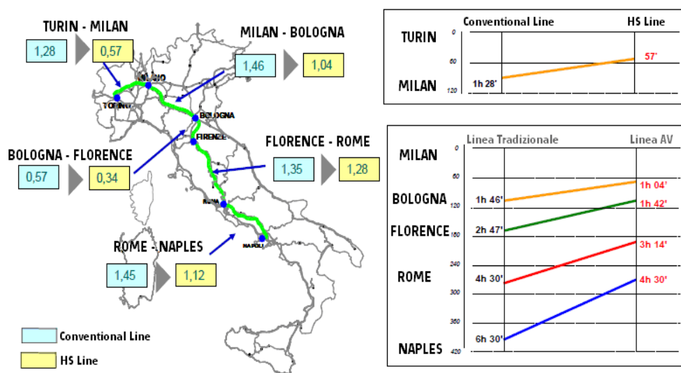
Figure 9: Journey time improvements on the HS/HC Italian line Milan-Naples
