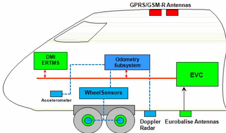
Figure 31: Simplified On-Board System
