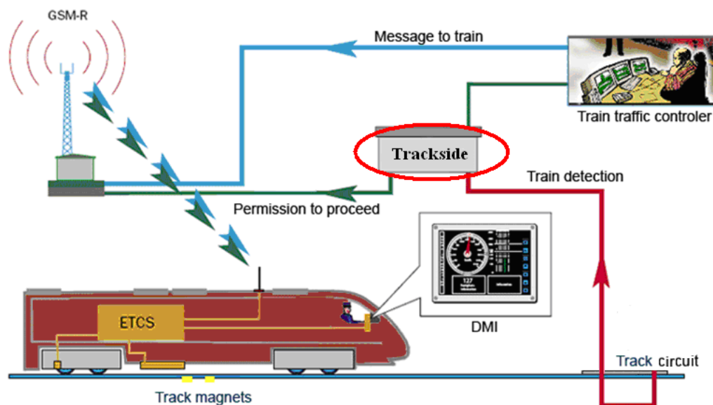
Figure 23: Communication of the trackside subsystem with other ERTMS L2 elements
