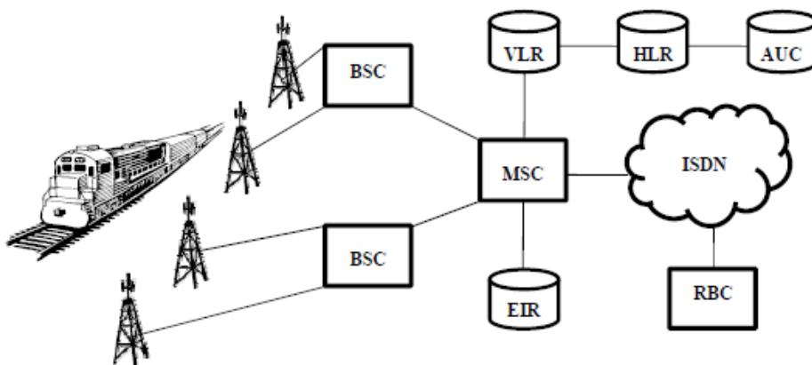
Figure 12: GSM-R Architecture
