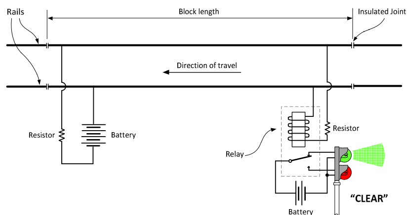
Figure 3: track circuit with unoccupied block
