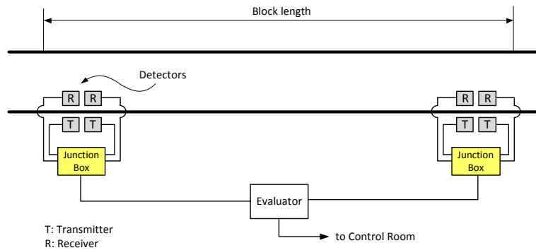
Figure 5: Schematic of Axle Counter system
