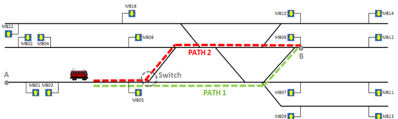
Figure 27: Two possible routes from A to B
