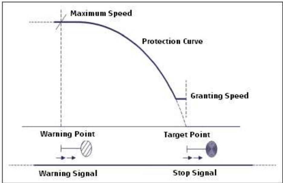
Figure 7: Safe Braking Model
