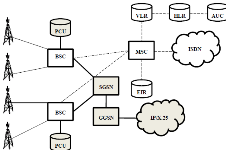
Figure 40: GPRS-R Architecture
