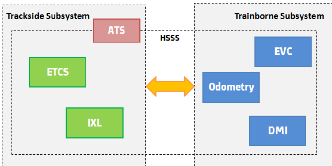
Figure 22: HS/HC railway transport system
