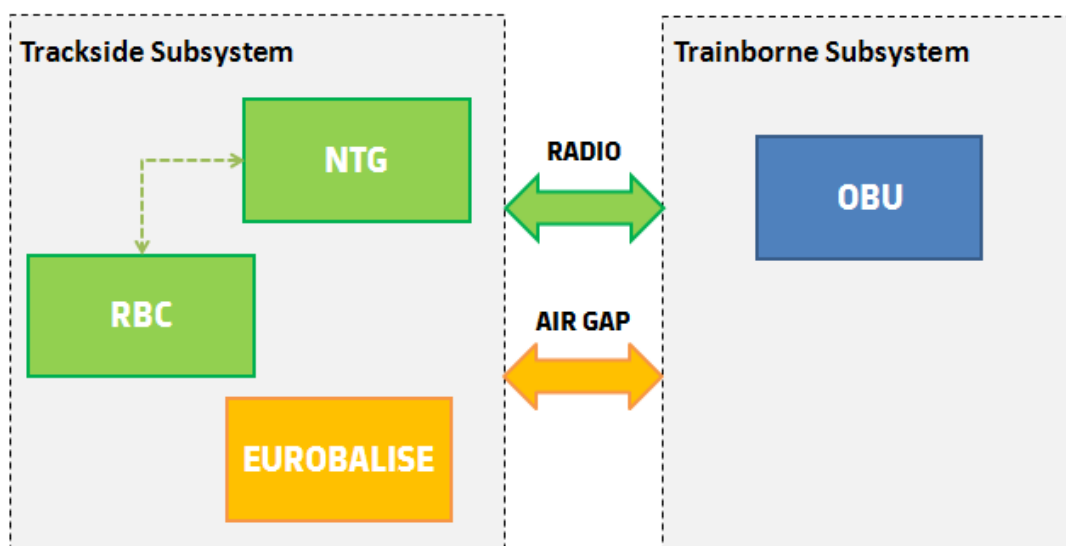
Figure 39: Interface between Trackside and Trainborne Subsystems
