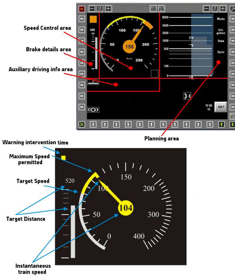
Figure 30: ETCS DMI monitor
