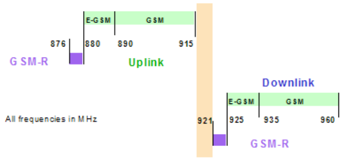
Figure 11: Frequency allocation in 900 MHz-Band
