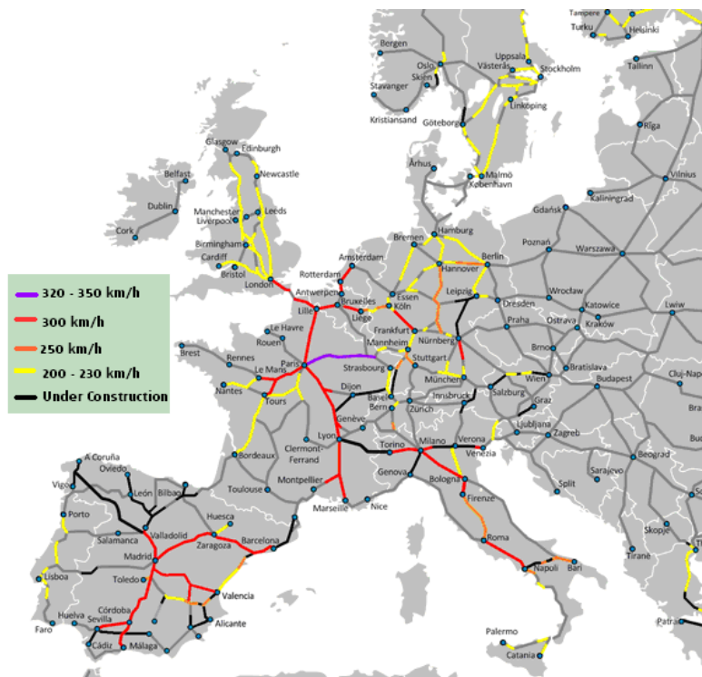
Figure 10: HS/HC railway European network
