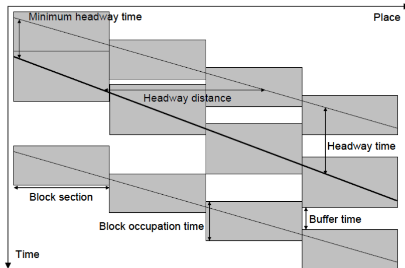
Figure 37: Rail capacity parameters
